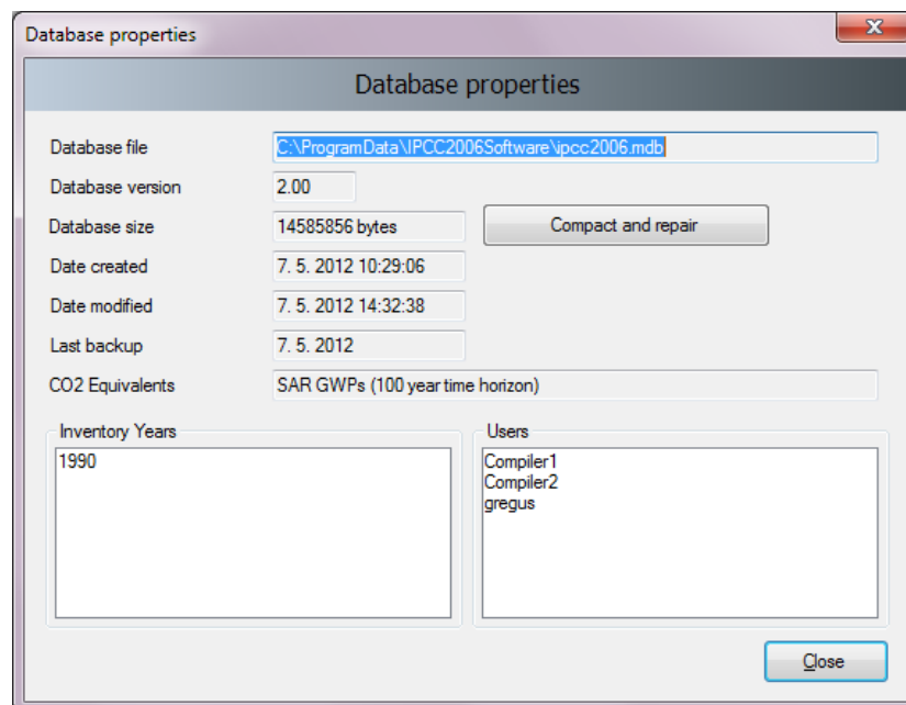
Figure 3.8 – Database properties
