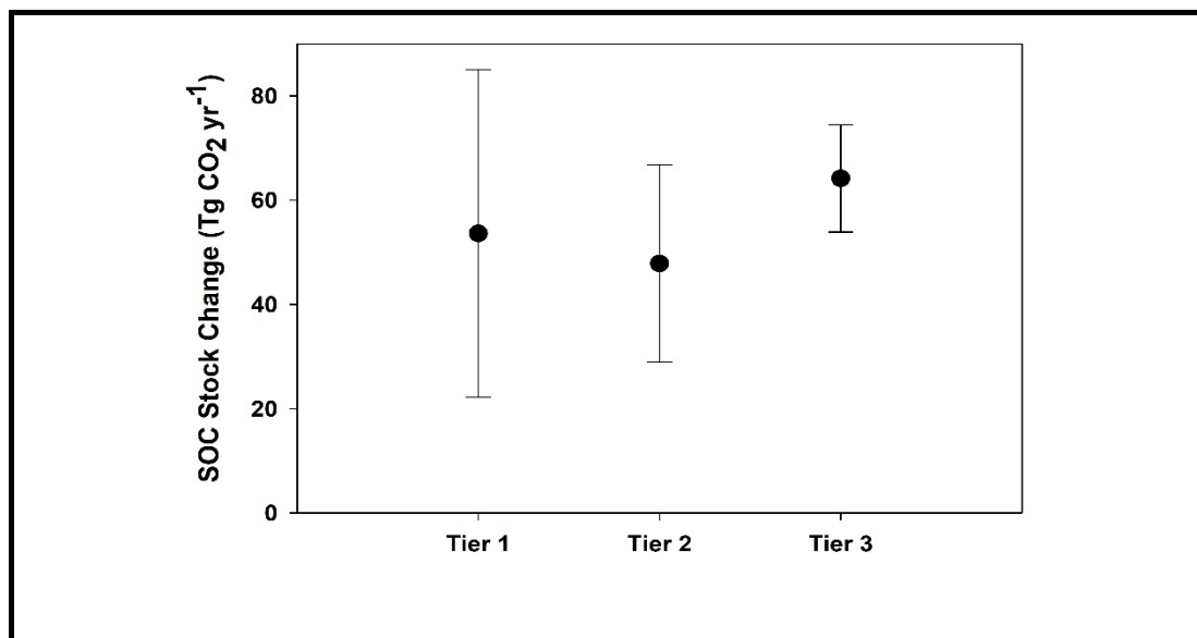
Figure 3.2a (New) Estimated soil organic C stock changes (Tg CO 2 eq. yr -1 ) and 95 percent confidence intervals for Tier 1, 2 and 3 methods as applied in the national greenhouse gas inventory for the United States (US EPA 2017)
