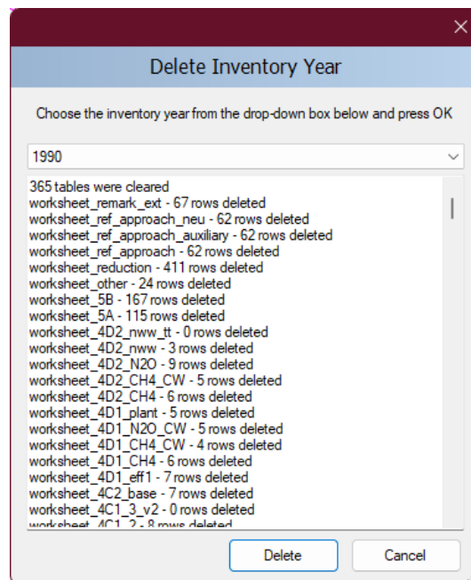
Figure 3.24 – Deleting inventory
