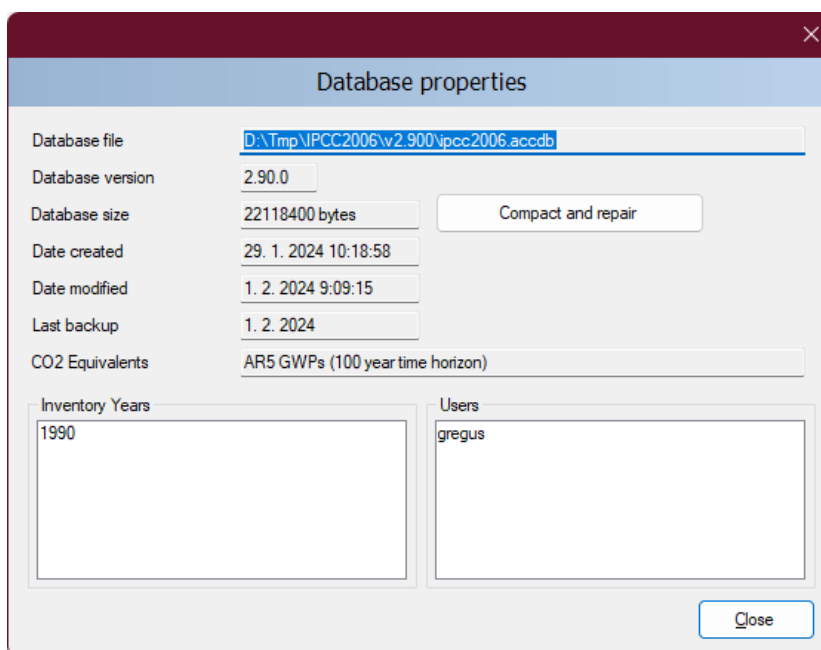
Figure 3.8 – Database properties
