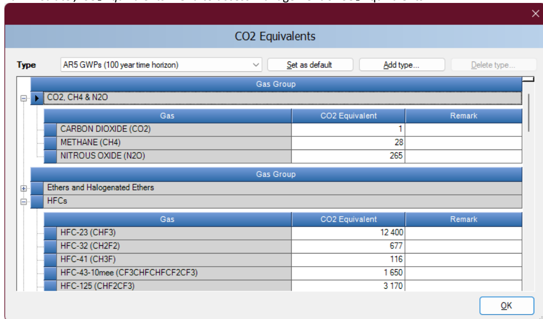
Figure 2.5 – CO 2 Equivalentents
